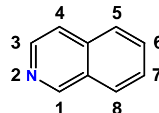
isoquinoline
